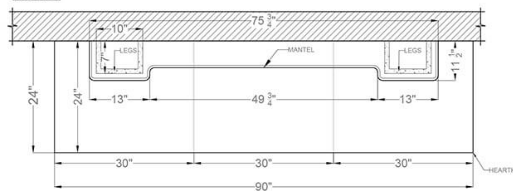
TOP VIEW
