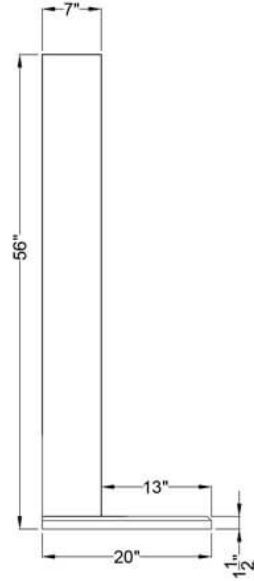
SIDE VIEW
